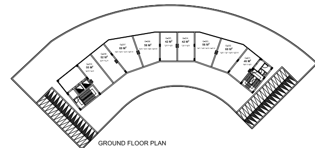
GROUND FLOOR PLAN ORO OBOUR CITY MALL 2
