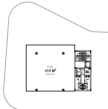
FIRST FLOOR PLAN ORO OBOUR CITY MALL 1
