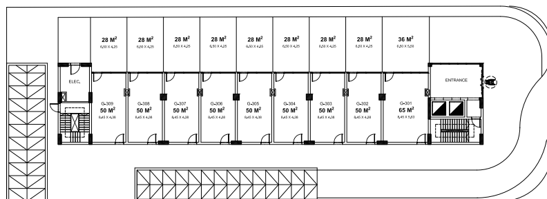
GROUND FLOOR PLAN ORO OBOUR CITY MALL 3
