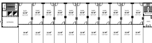
GROUND FLOOR PLAN ORO OBOUR CITY MALL 5
